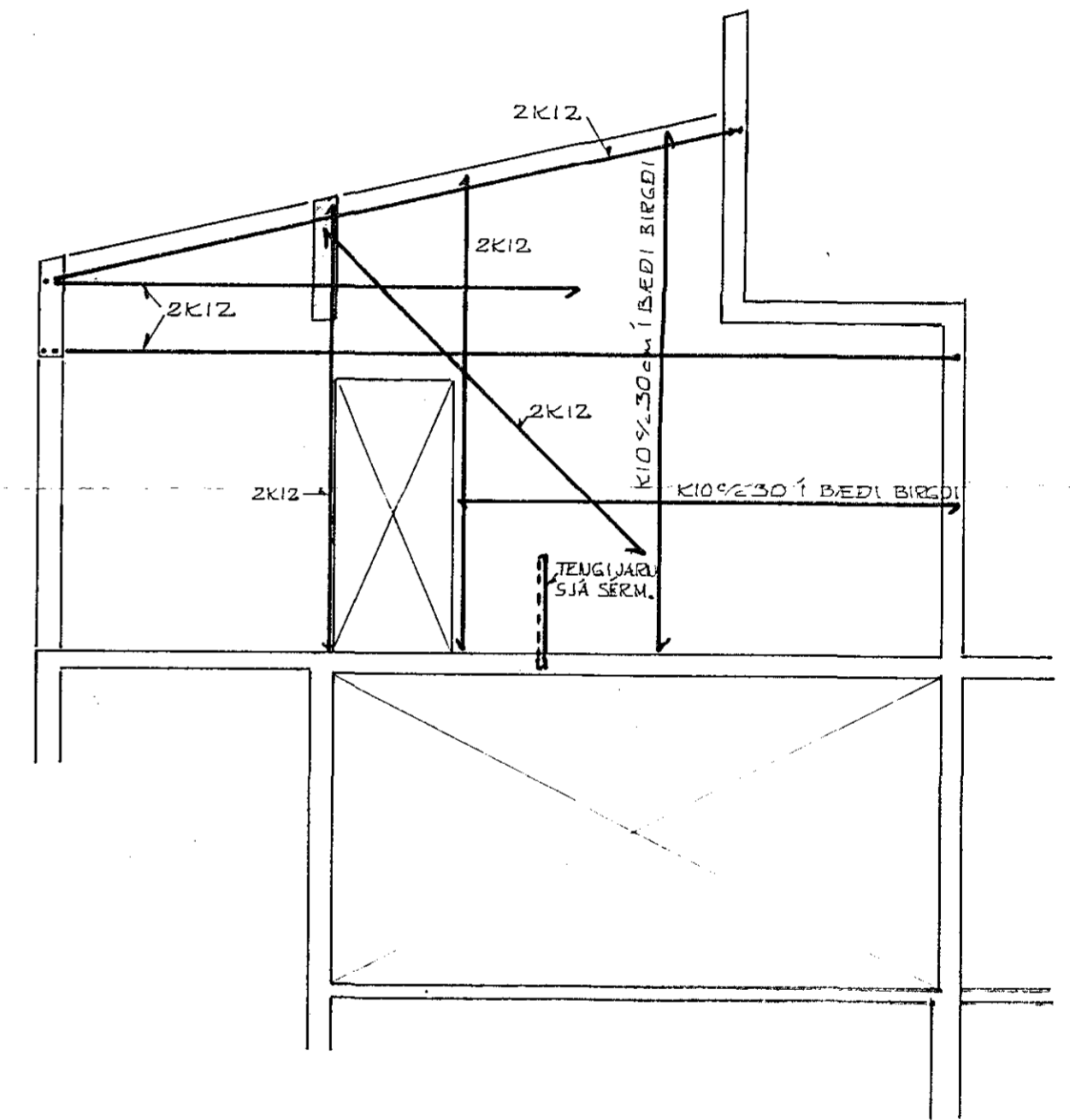
SNID F-F
