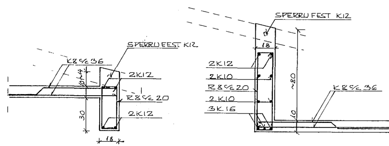
SNID II-II 1:20
