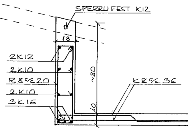
SNID II-II 1:20
