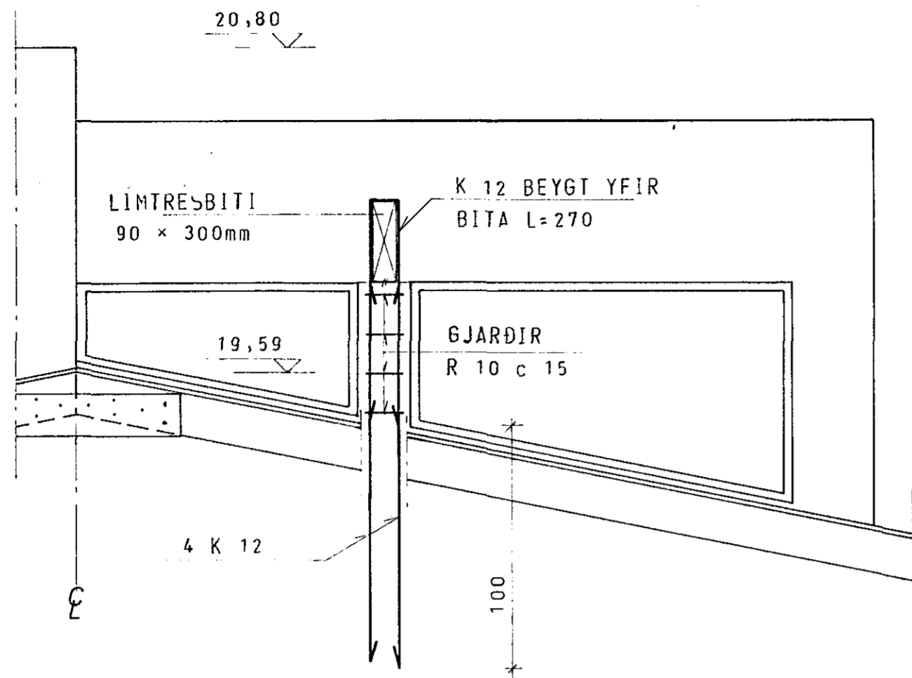
SNID K 1:20
