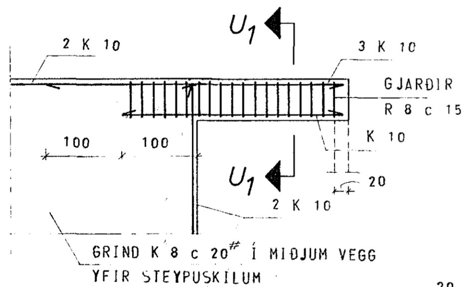
SNID U 1:50
