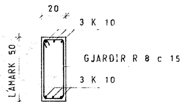
SNID U 1 1:20
