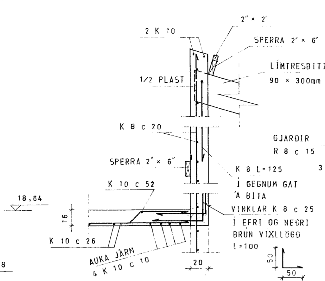
SNID R 1:20
