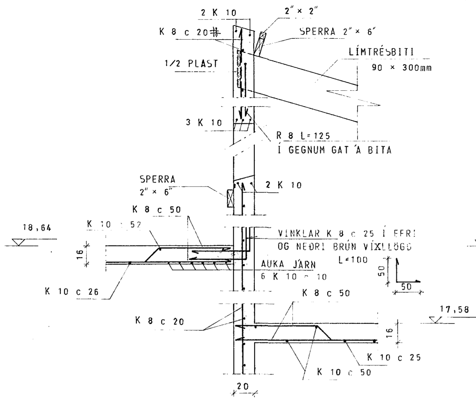
SNID P 1:20
