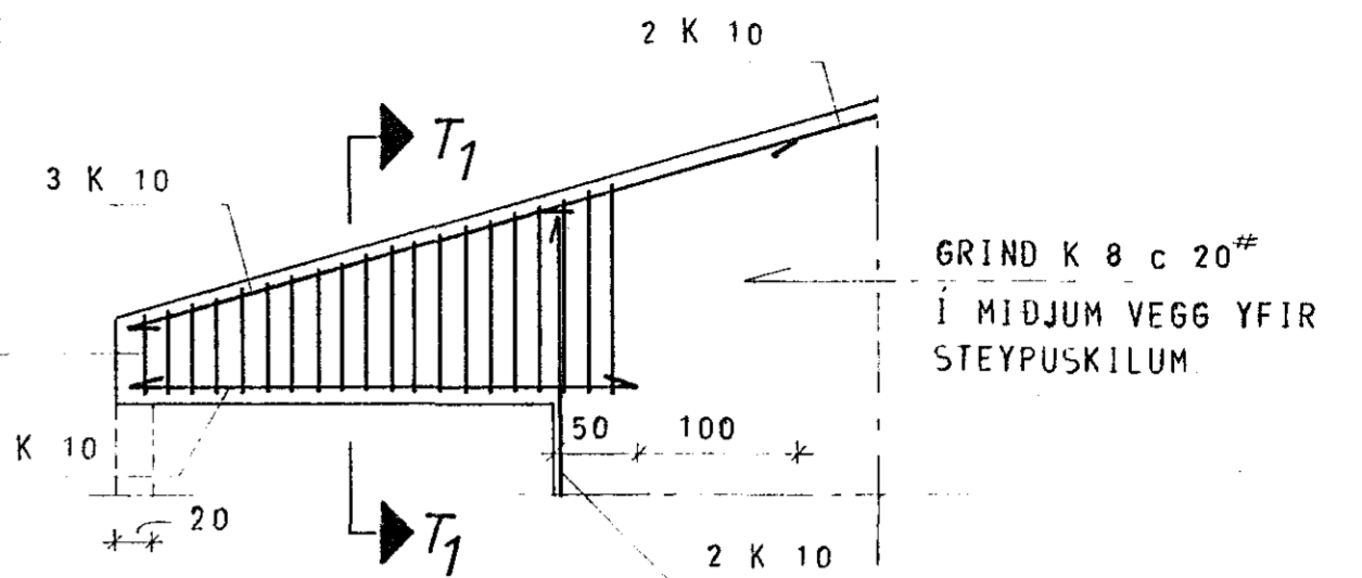
SNID T 1:50
