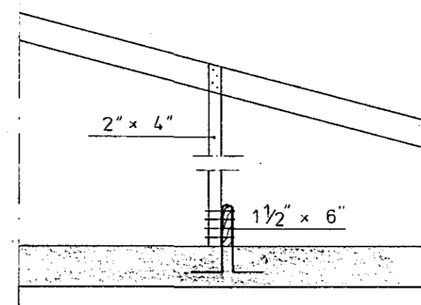
SNID B 1:20
