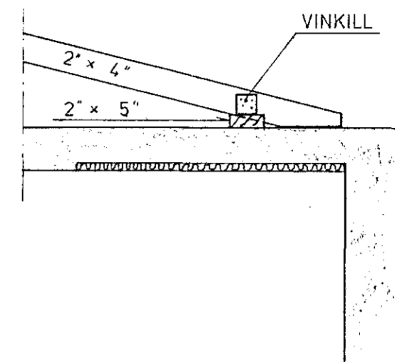
SNID C 1:20
