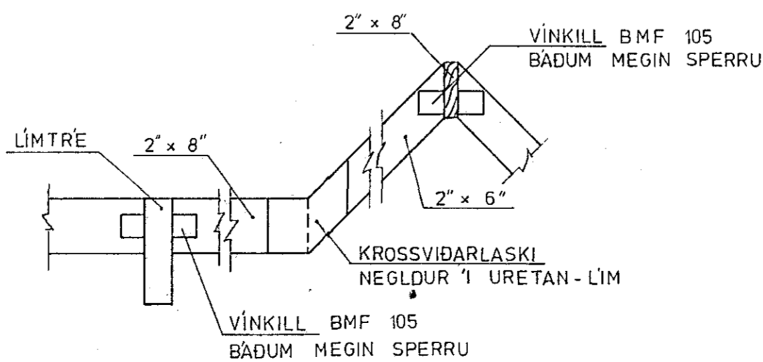
SNID F 1:20
