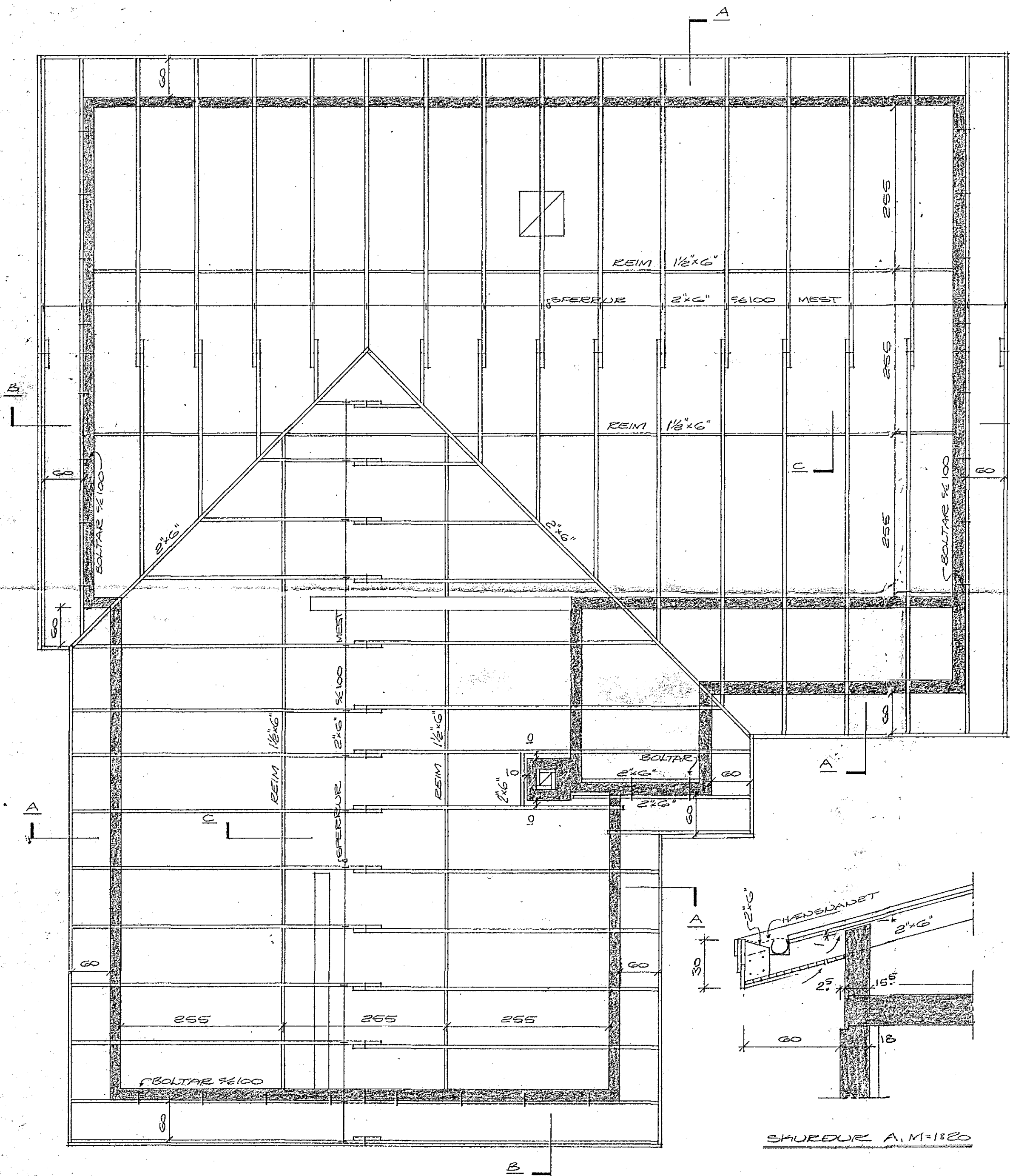
GRUNNMÝND, M=1:850
