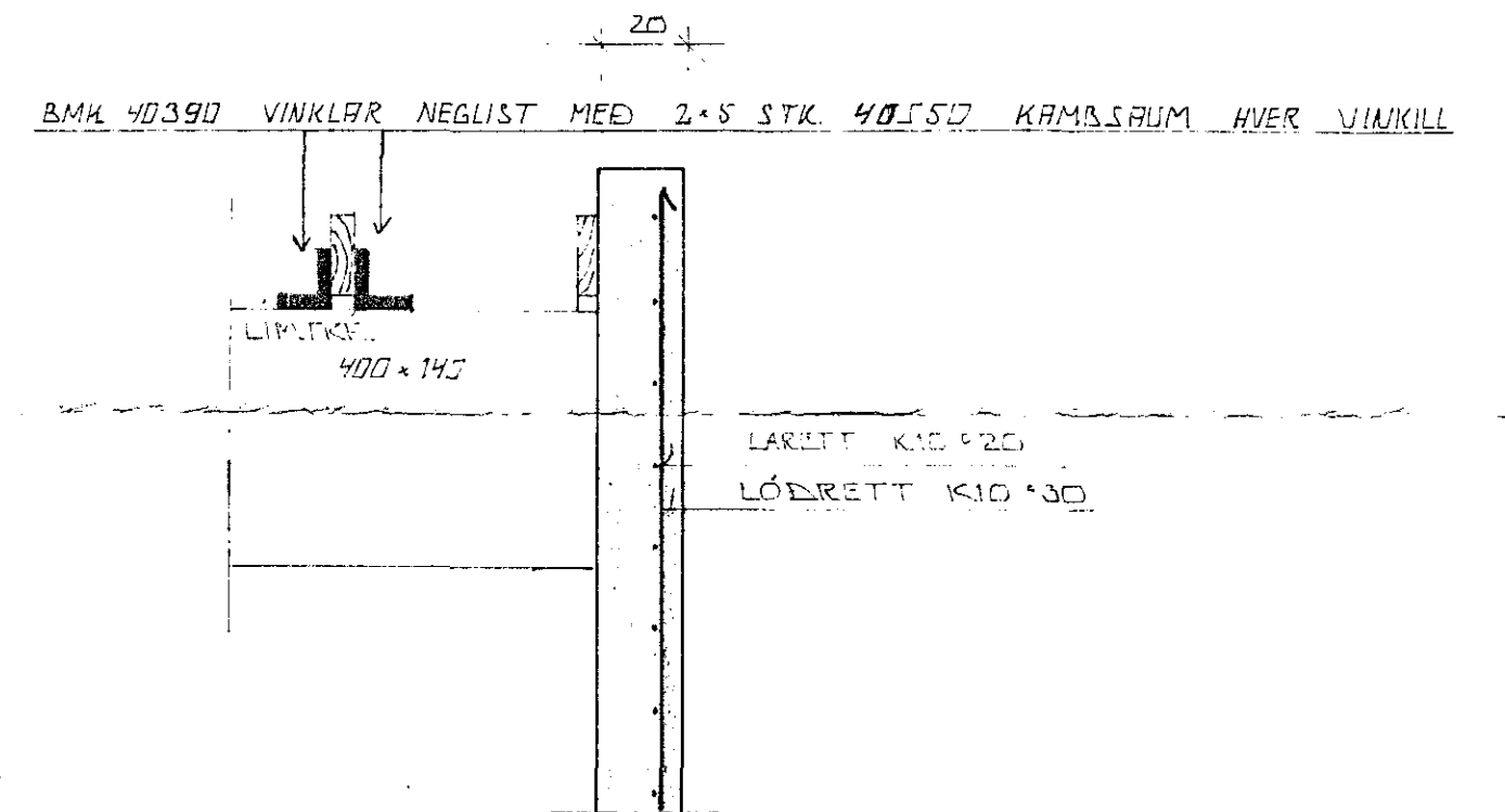
SNID C - C \times 1:20
