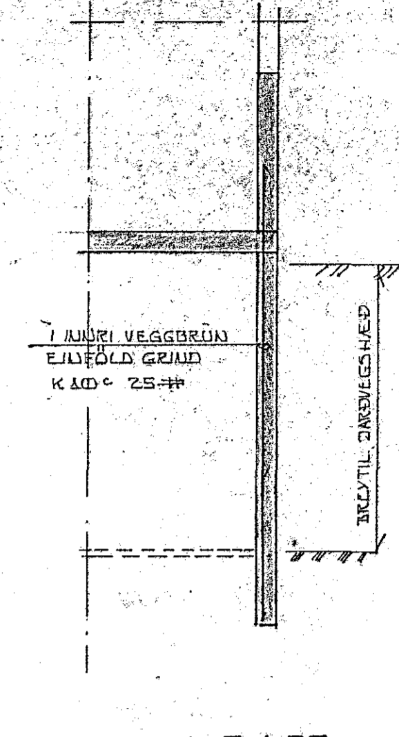
SNID C-C 1:50
