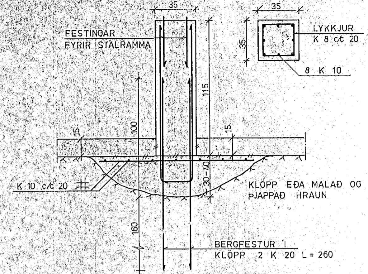
SNID A 1:20
