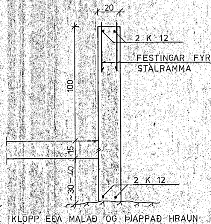
SNID C 1:20
