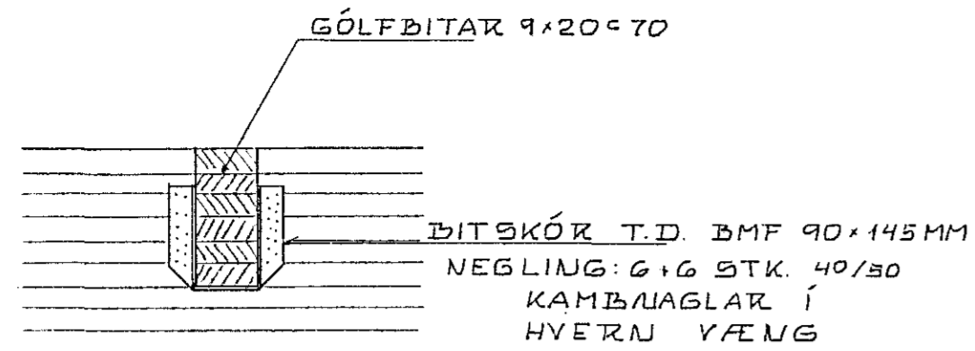
SNID IIa - IIa 1:10
