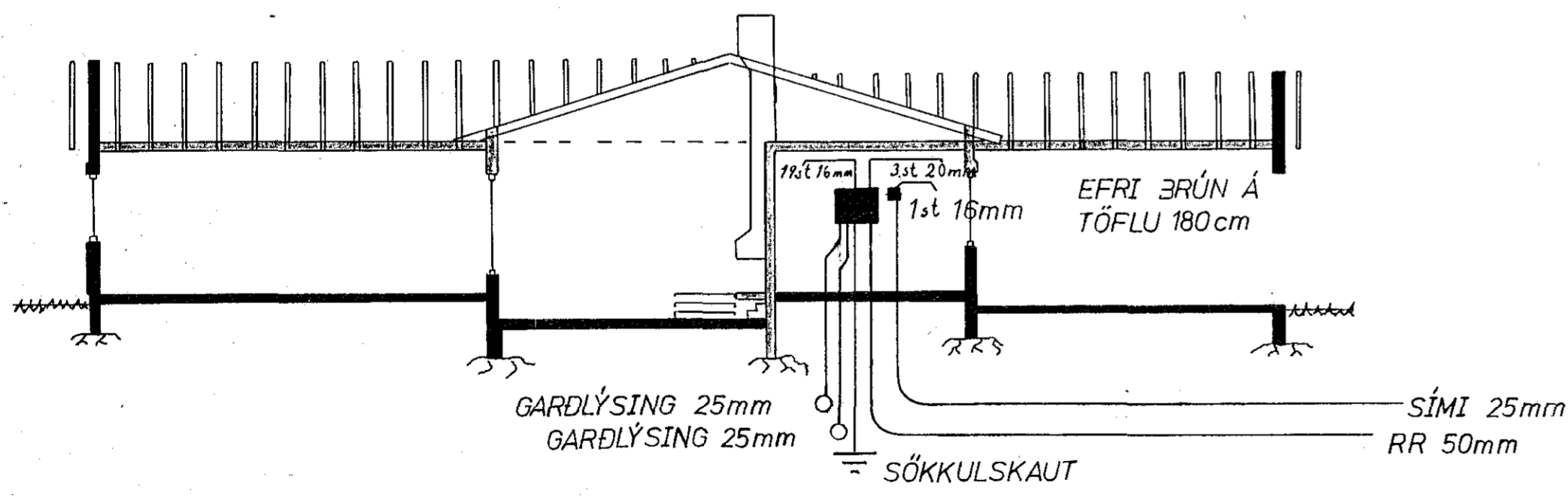
SNID M=1:100
