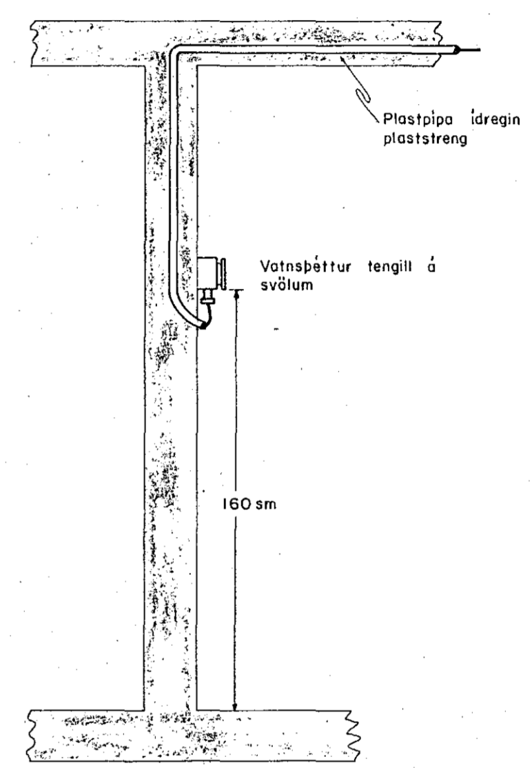
SNID C - C M = 1 : 20
