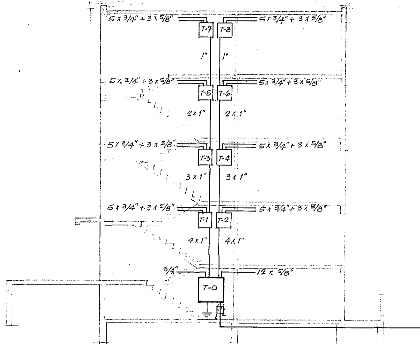
SNEIÞING - MKV = 1:100
