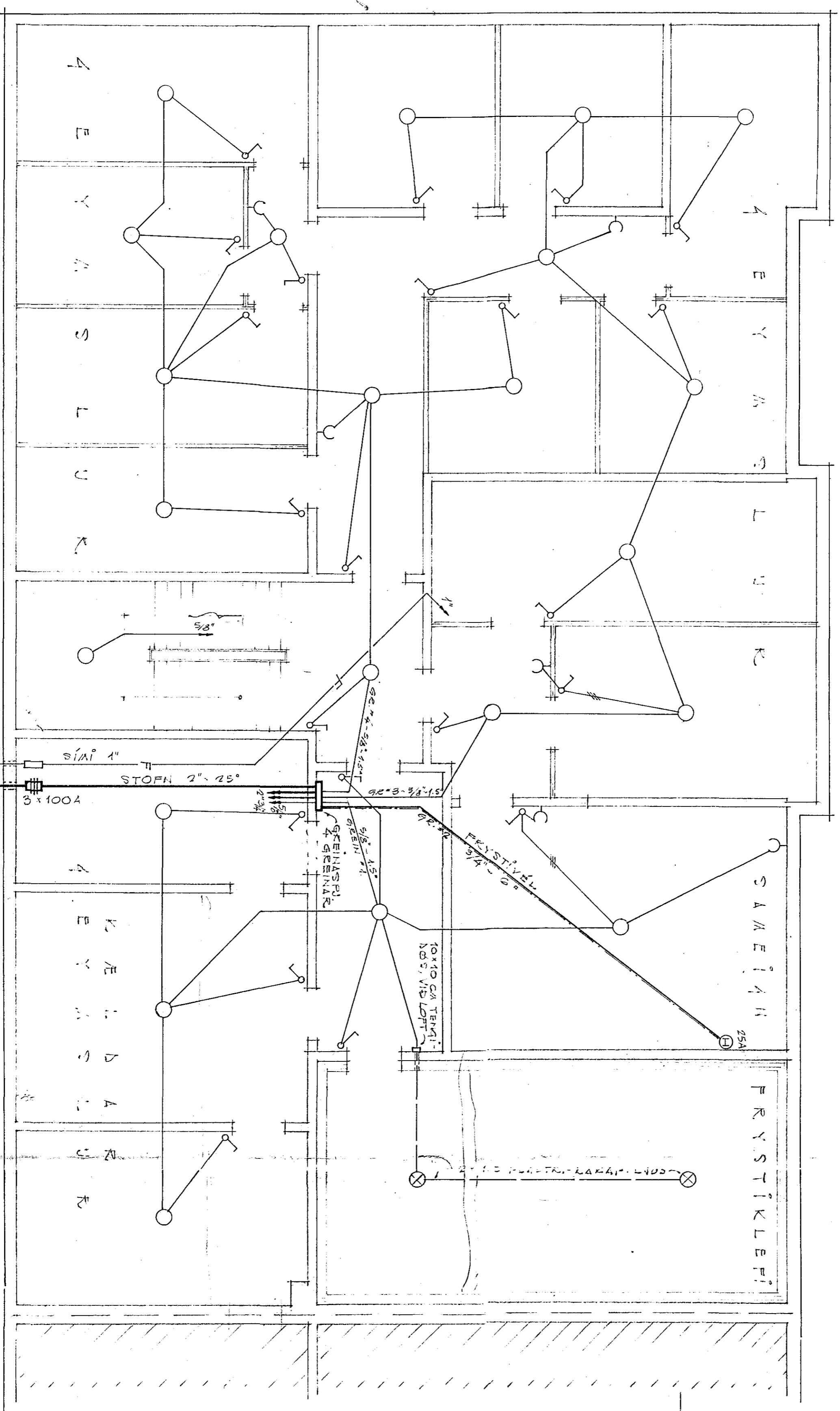
NEARI KJALLARI (NR. 100) M = 1:50
