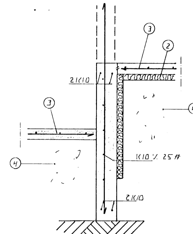
SNID 3, 1:20
