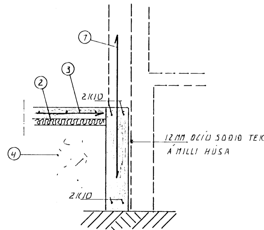
SNID 4, 1:20
