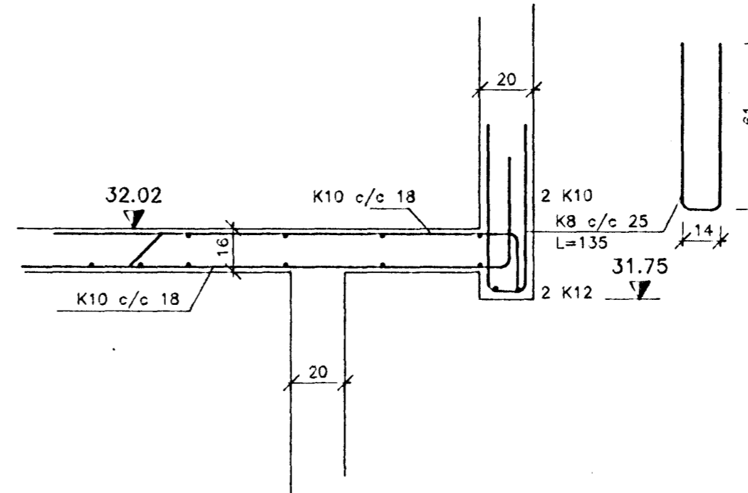
SNID 11-11 1:20
