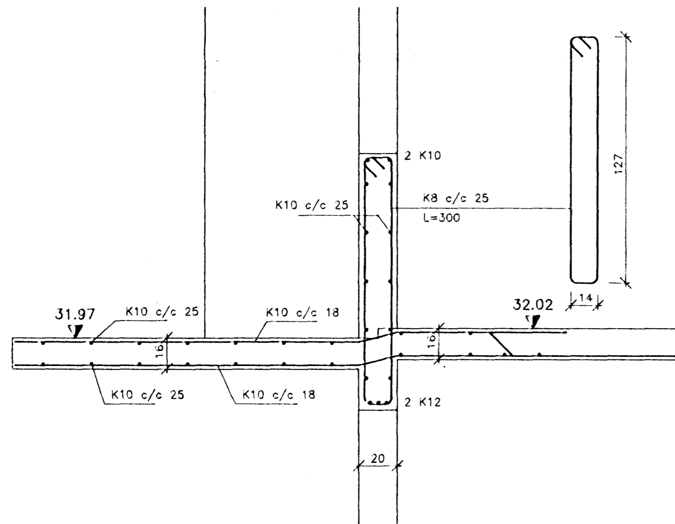
SNID 12-12 1:20
