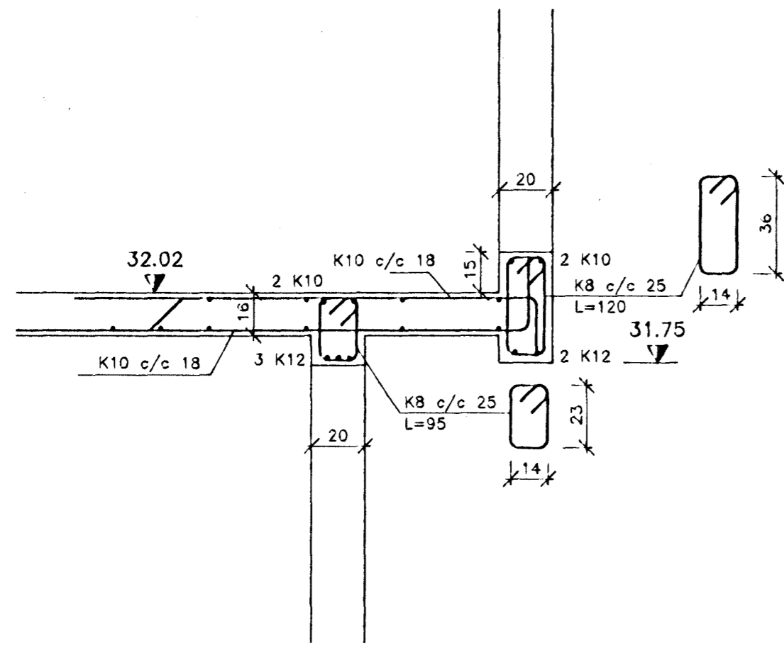
SNID 10-10 1:20
