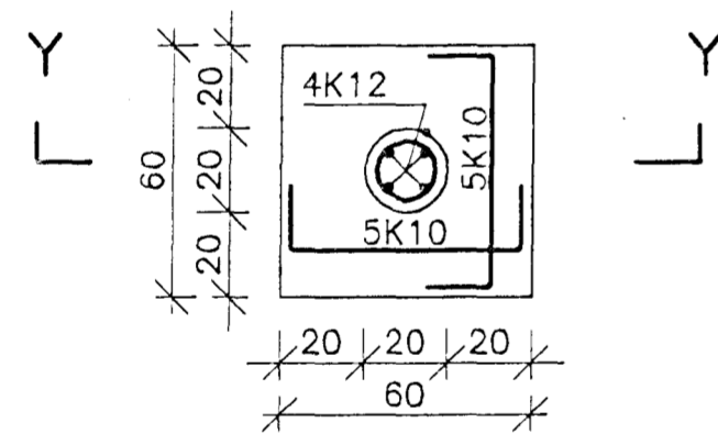
UNDIRSTADA U2 1:20
