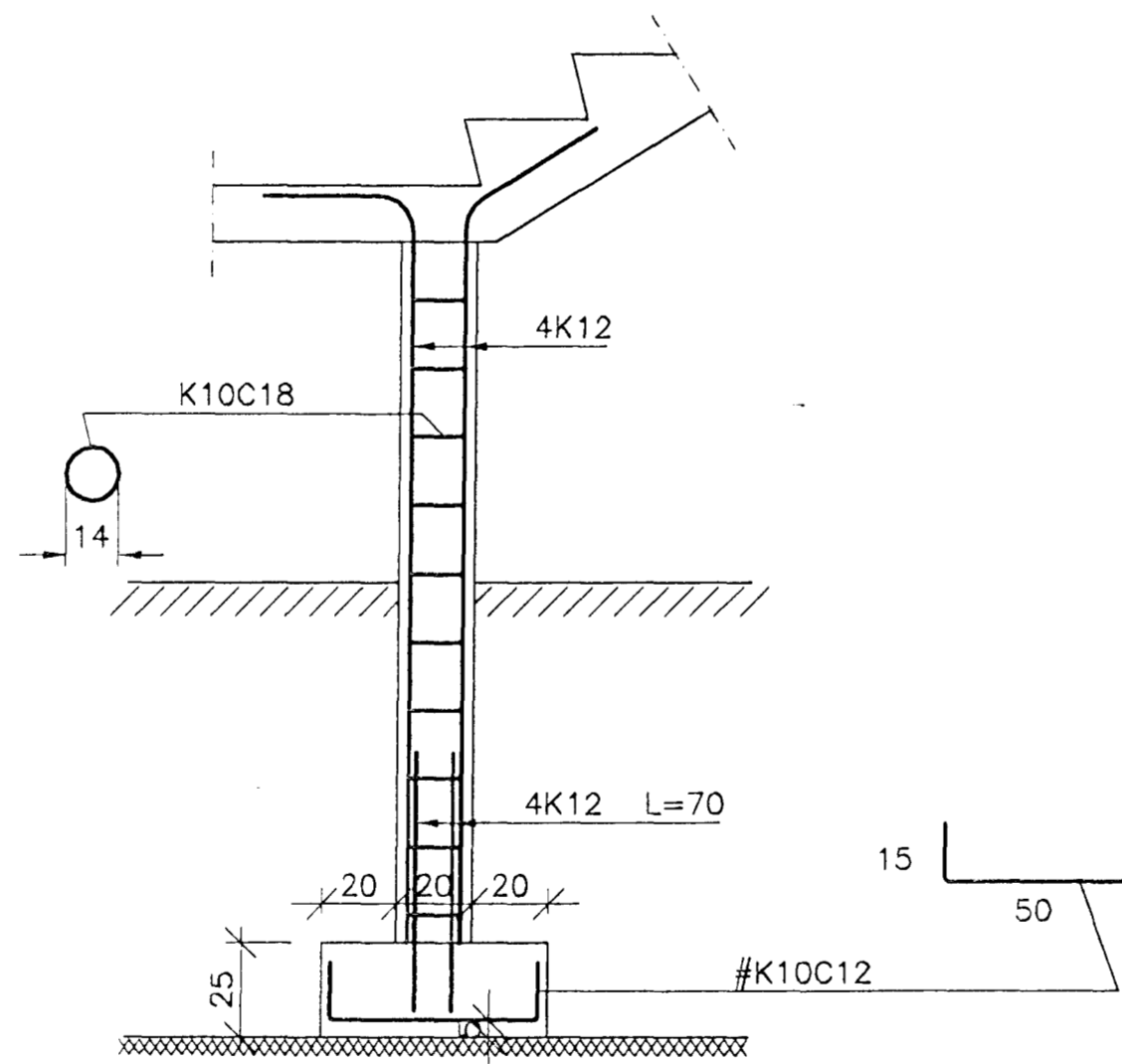
SNID Y-Y 1:20
