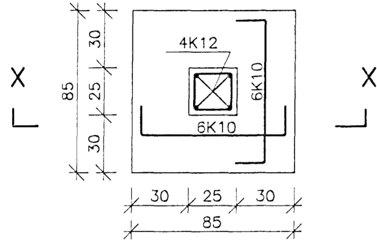
UNDIRSTADA U1 1:20
