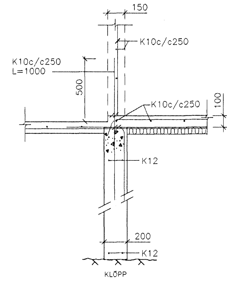
SNID 02, 1:20
