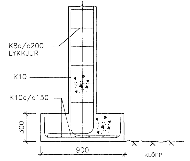
SNID 03, 1:20
