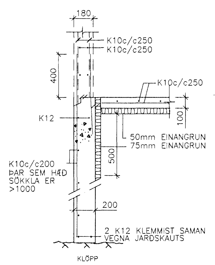
SNID 01, 1:20
