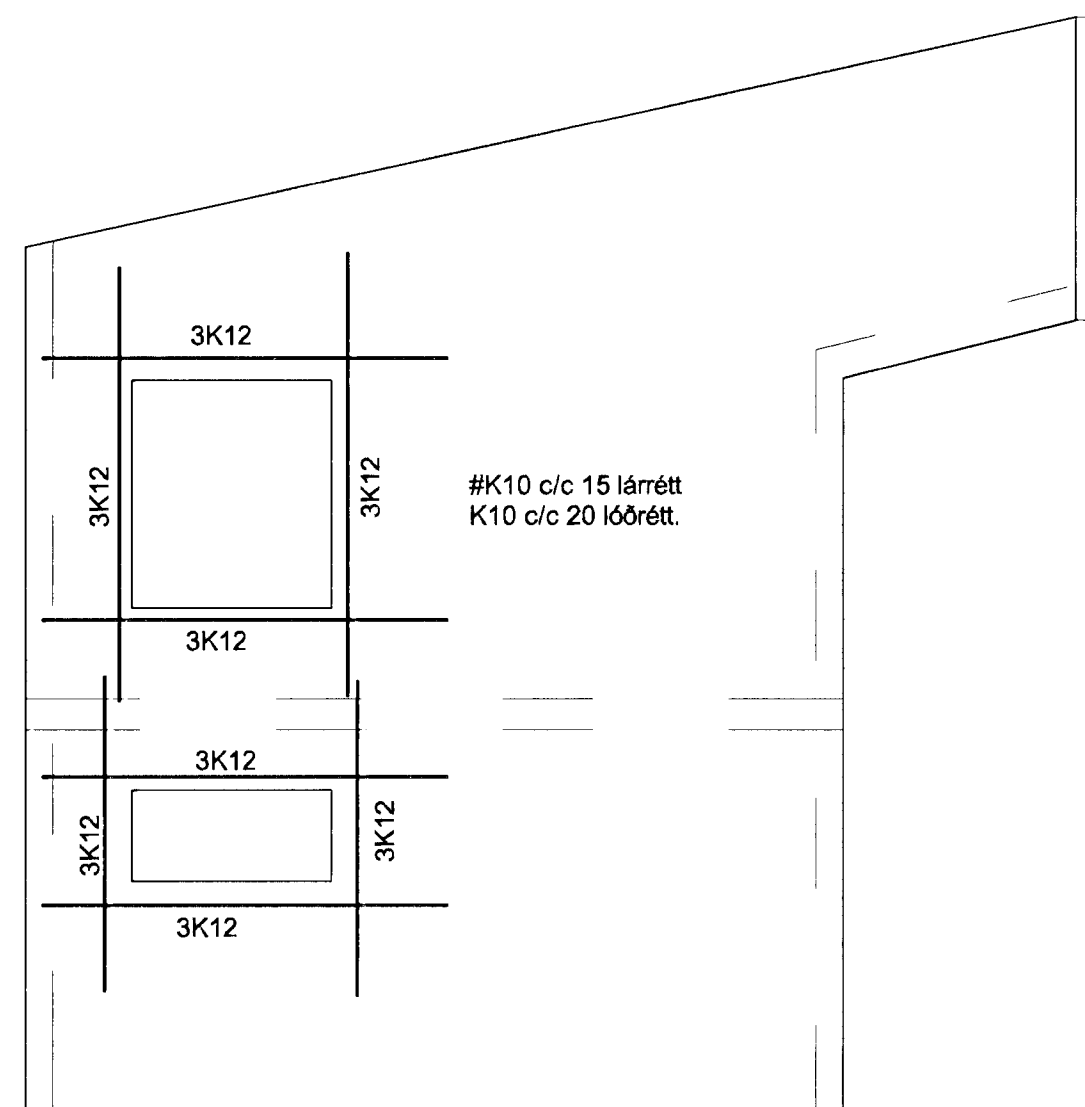
VEGGUR V9, MKV. 1:50
