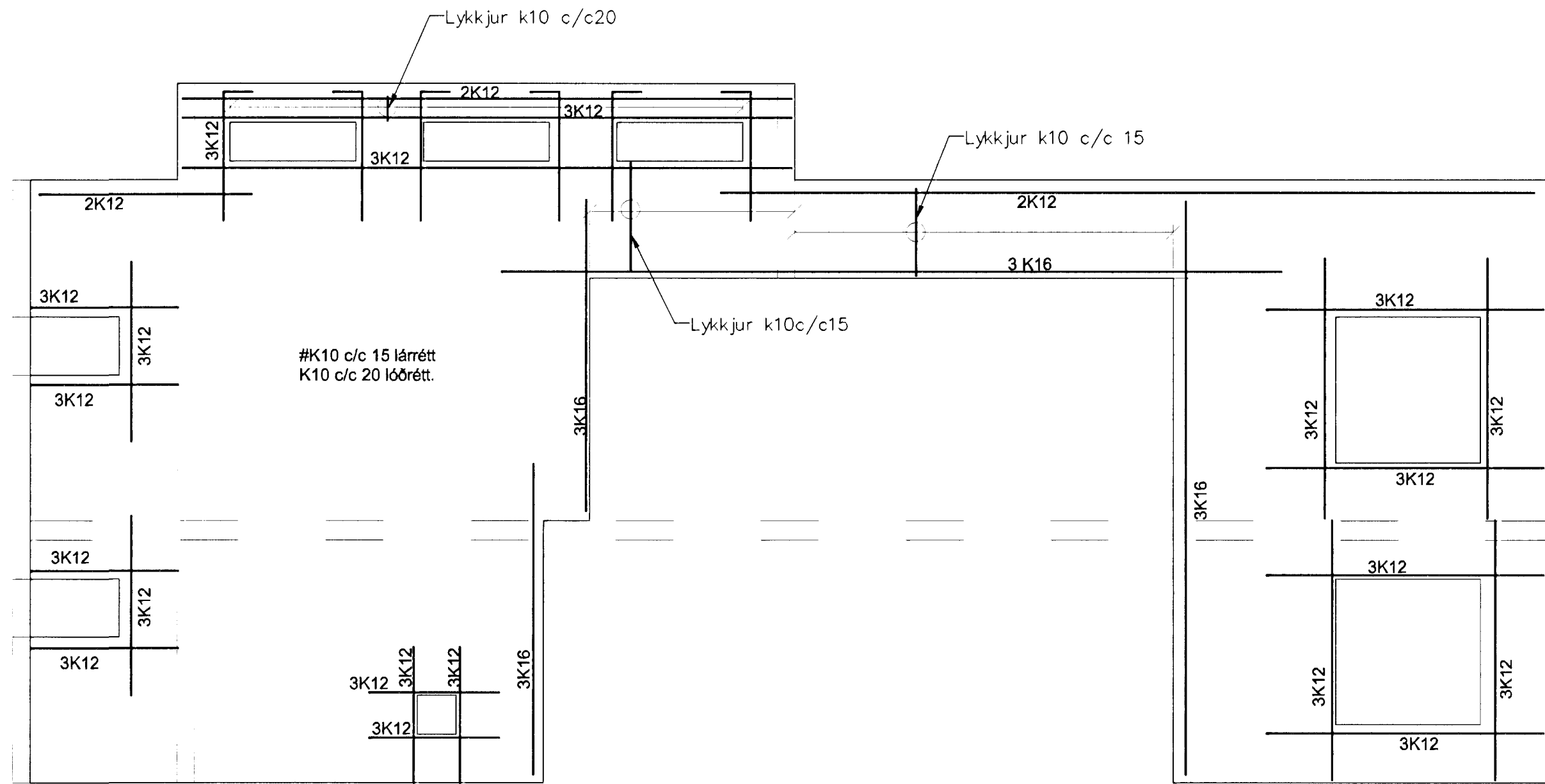
VEGGUR V11, MKV. 1:50
