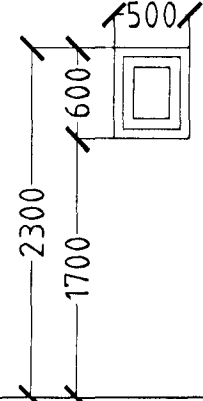
1 STK. V/S.
