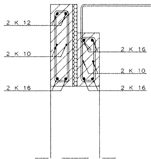
SNID -E 1:10
