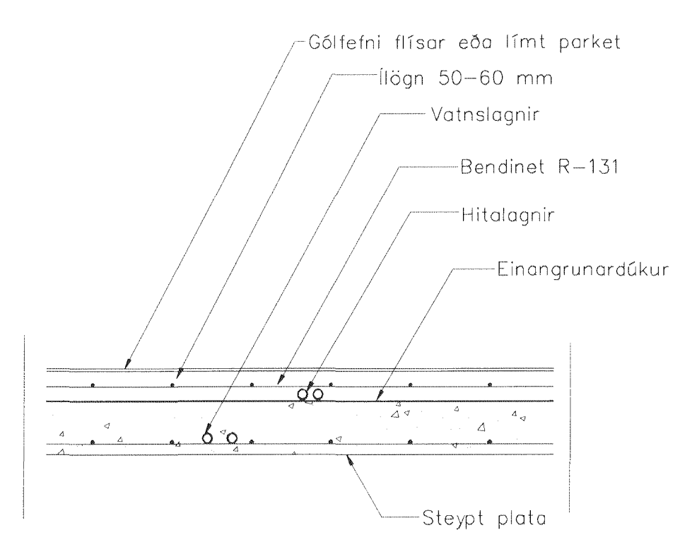
LAGNIR, SNID, 1:20
