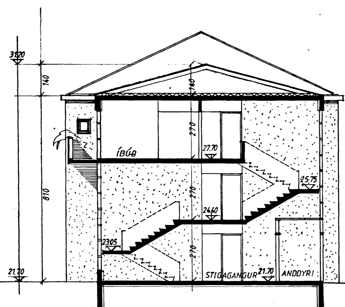
SNIB C-C
