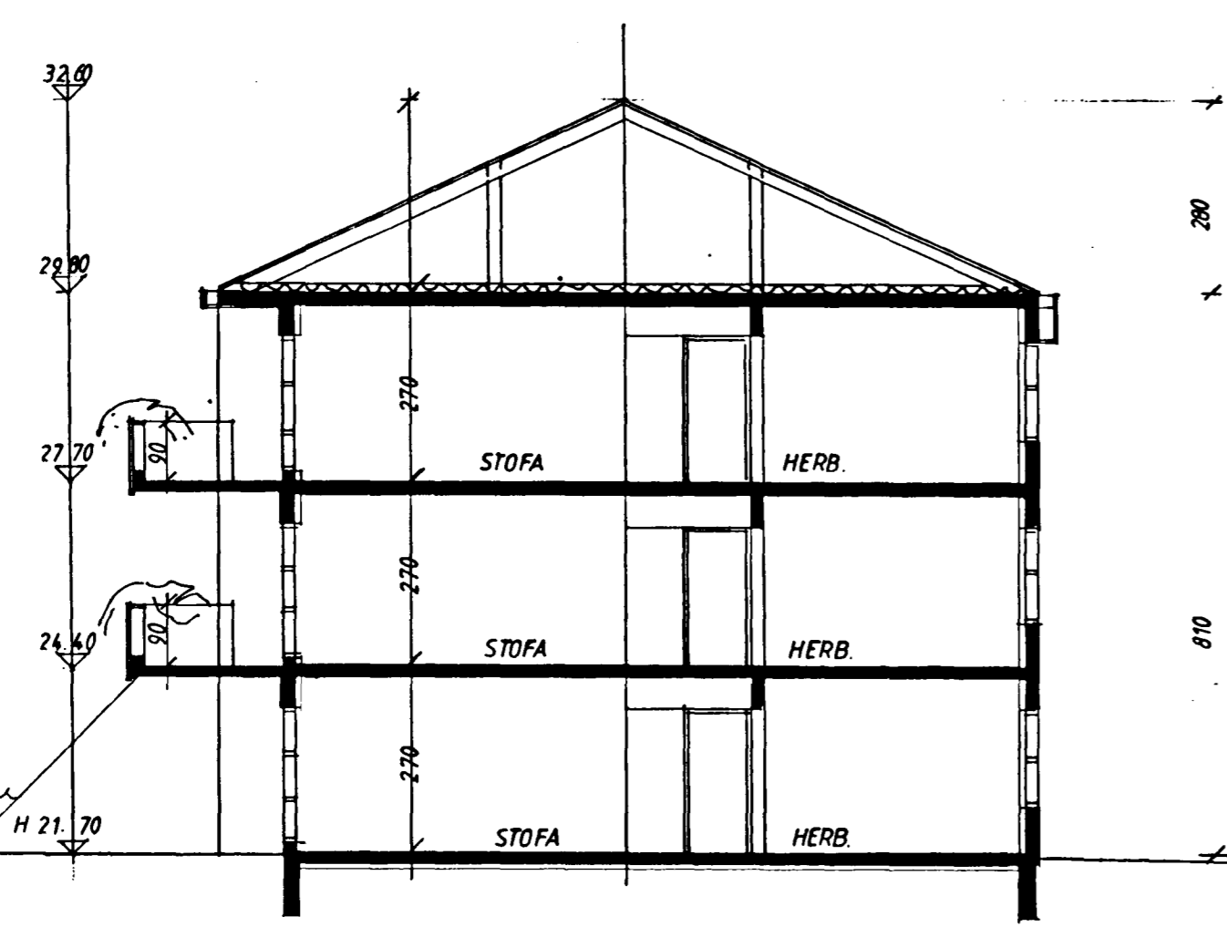
SNID B-B
