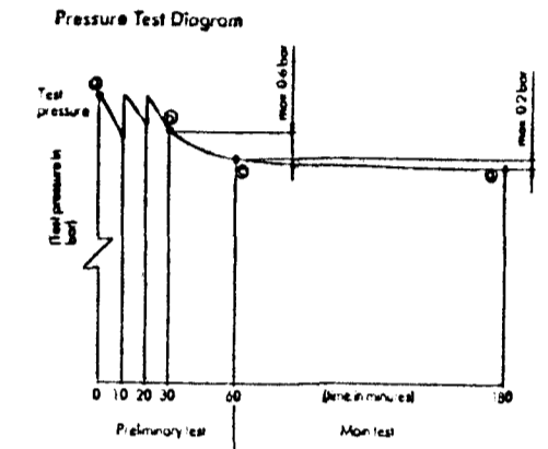
Pressure Test Diagram For an operating pressure of 10 bar, a test pressure of 15 bar should be used
