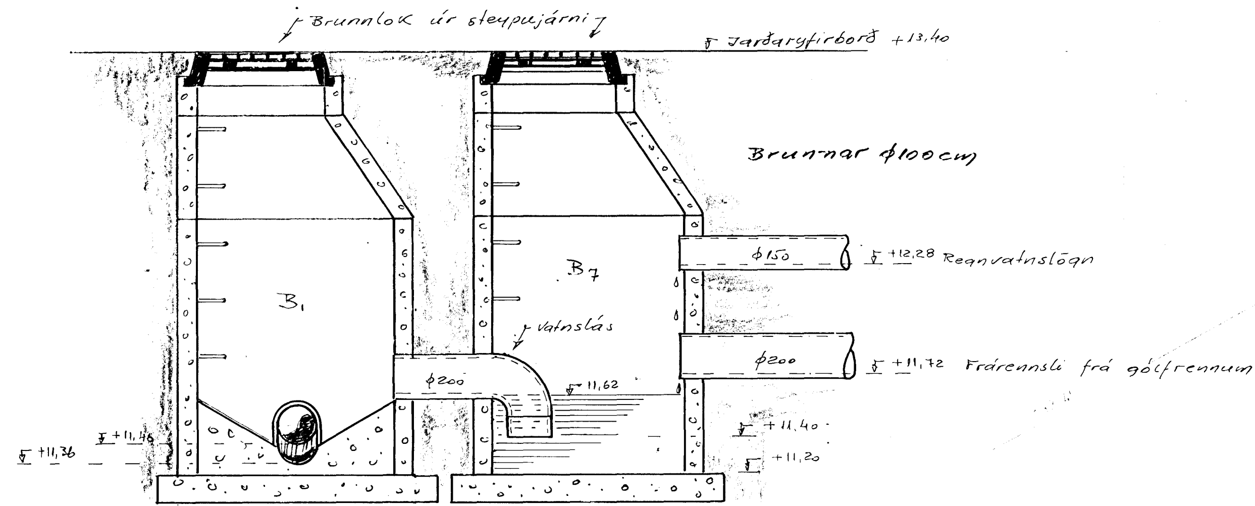
Tenging brunna MKV 1:20
