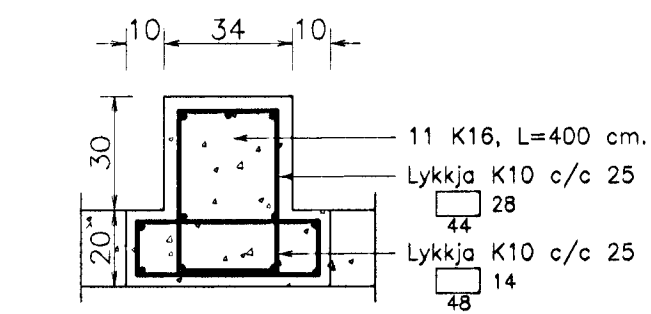
S2.2. Sála S2.2. 1:20. 8 | 9
