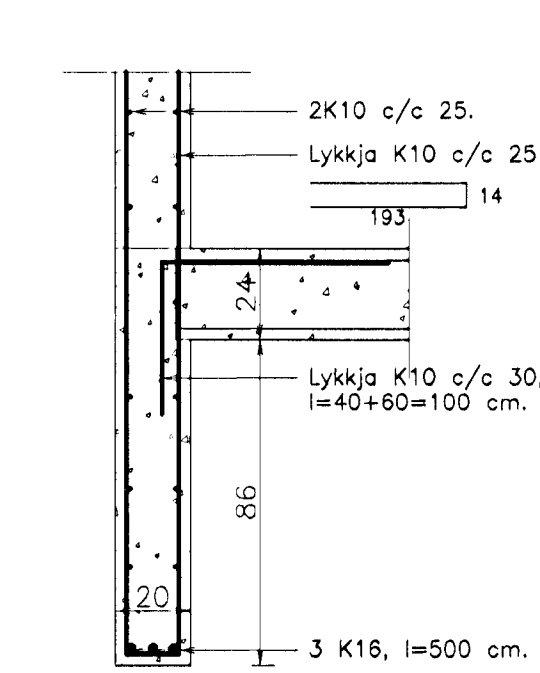
B1.3. Biti B1.3. 1:20.
