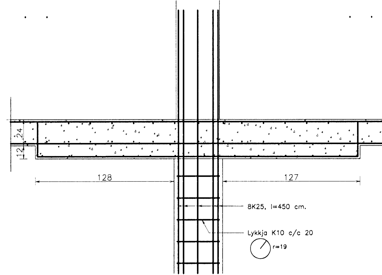
S1.3. Sála S1.3. 1:20.
