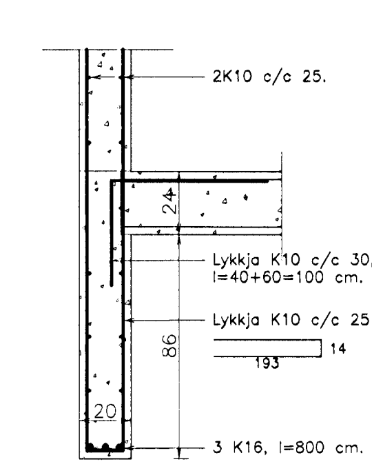
B1.2. Biti B1.2. 1:20.
