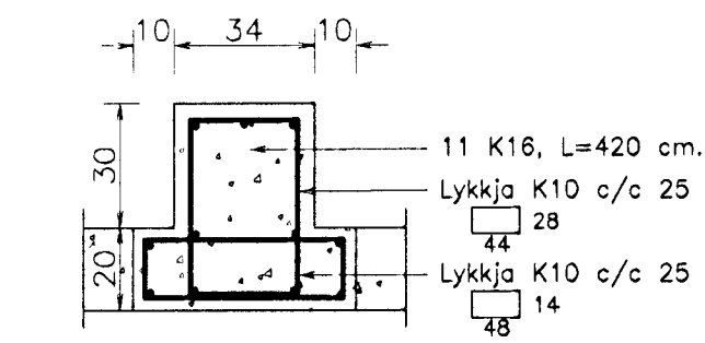
S1.2. Ógla S1.2. 1:20.
