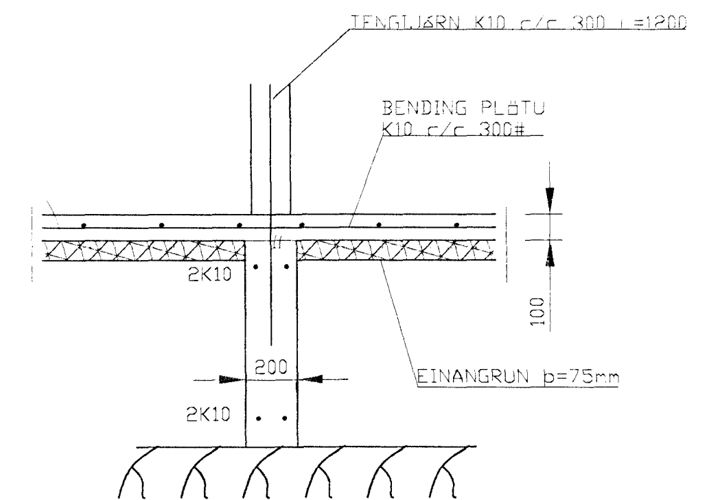
SNID 2, 1:20
