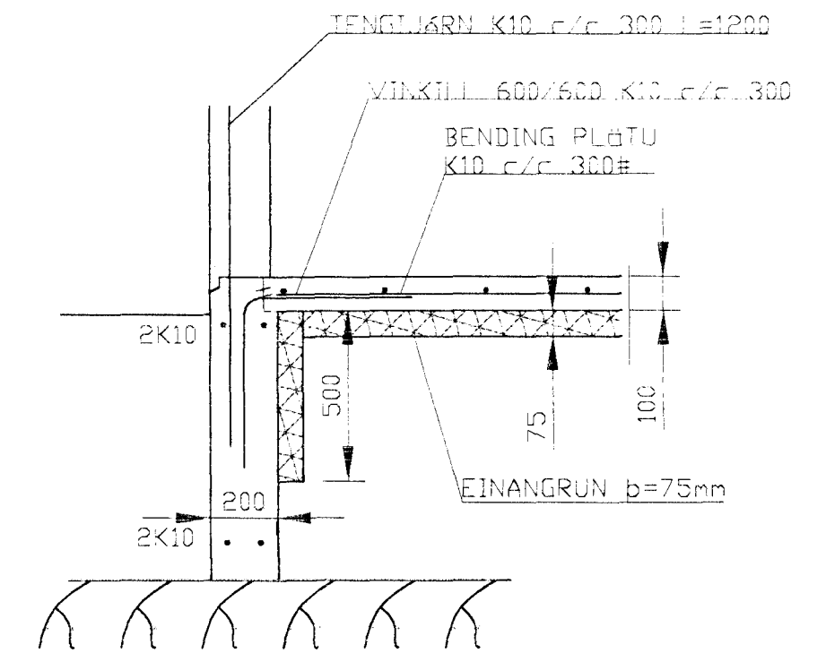
SNID 1, 1:20
