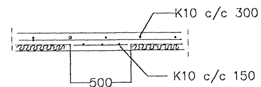
SNID 2, 1:20
