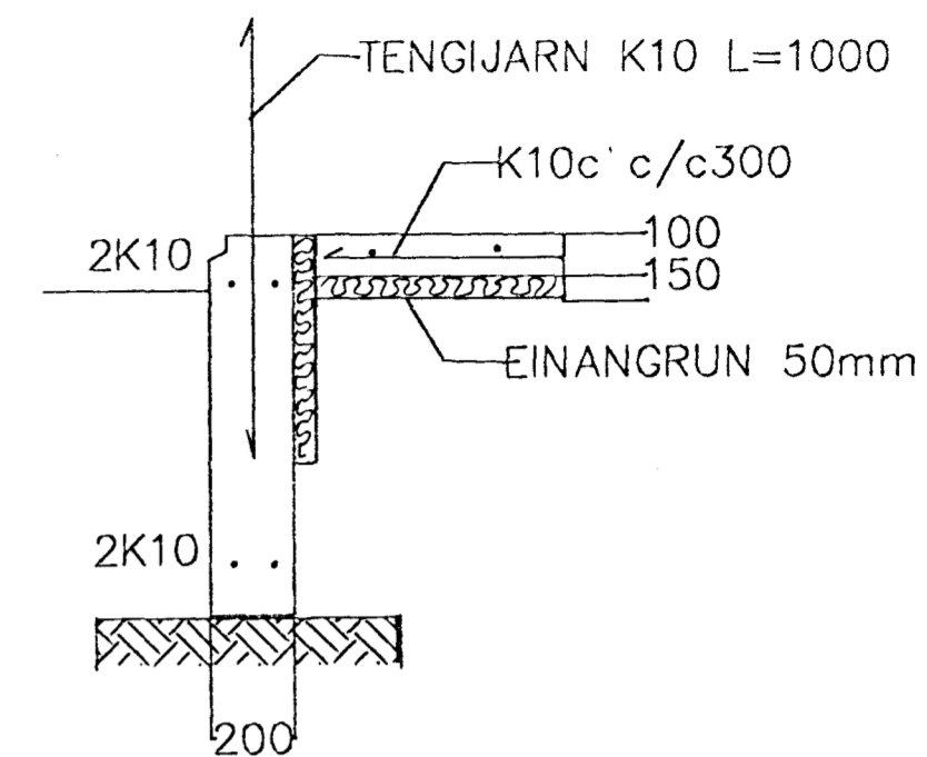
SNID 1, 1:20
