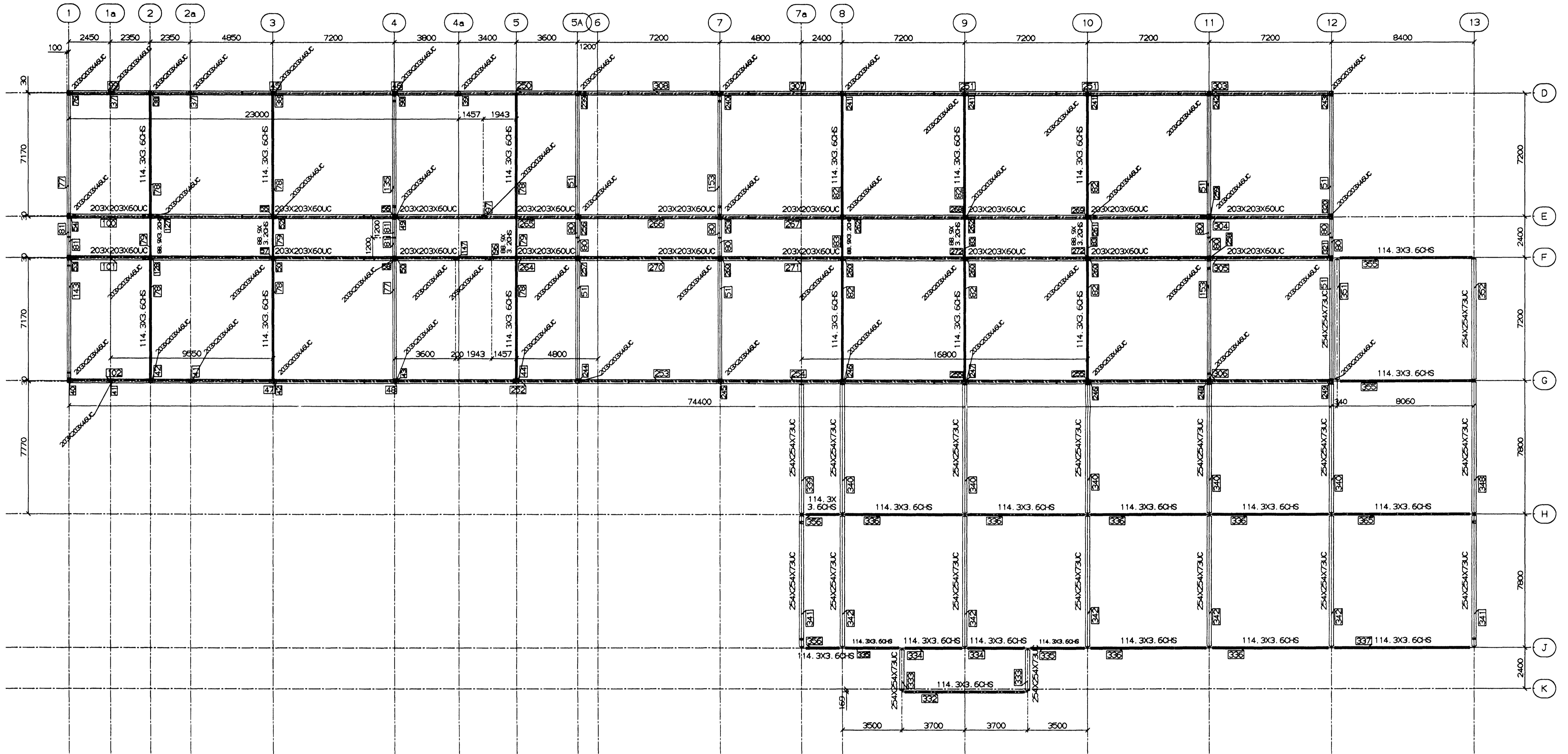
ROOF PLAN HOT ROLLED (EXCEPT COLUMNS) 203X203X46UC U.N.O.
