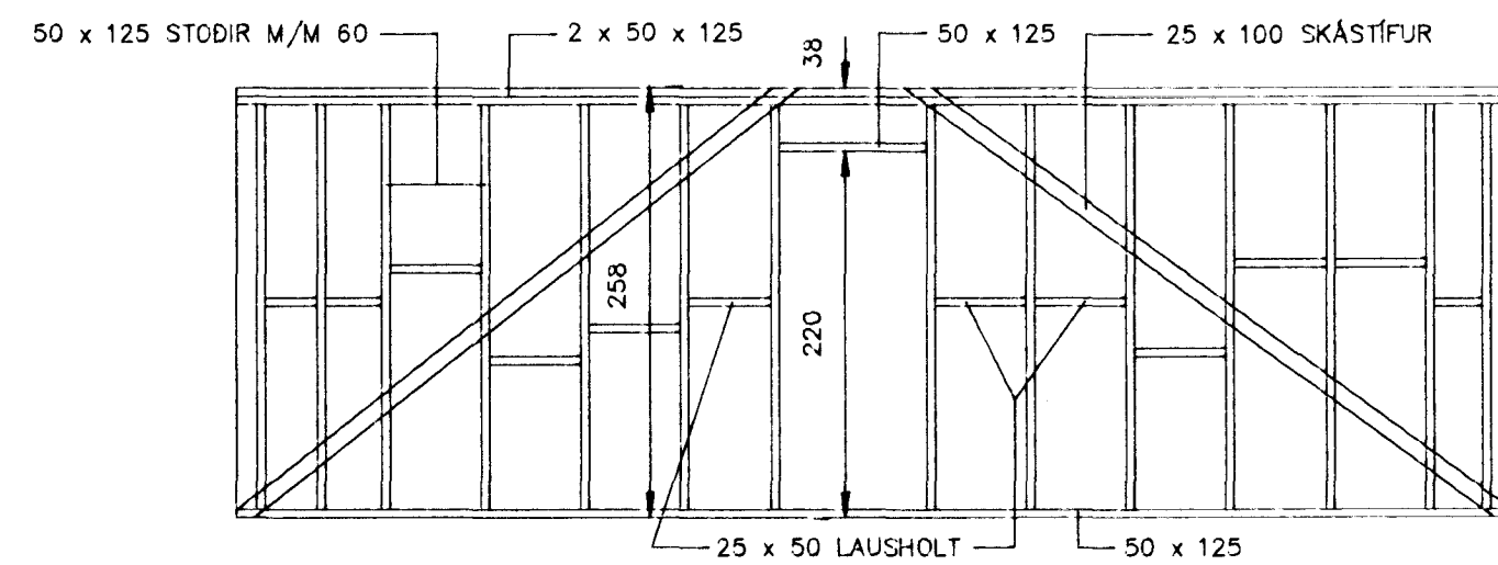
AUSTURHLID, M=1:50
