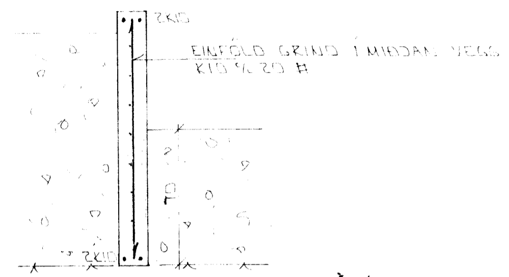
SNID 7 x 1:20
