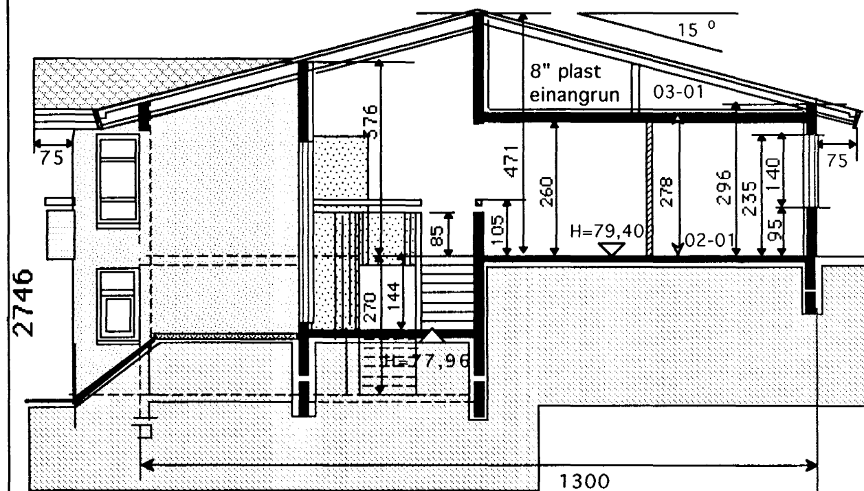
SNID B-B
