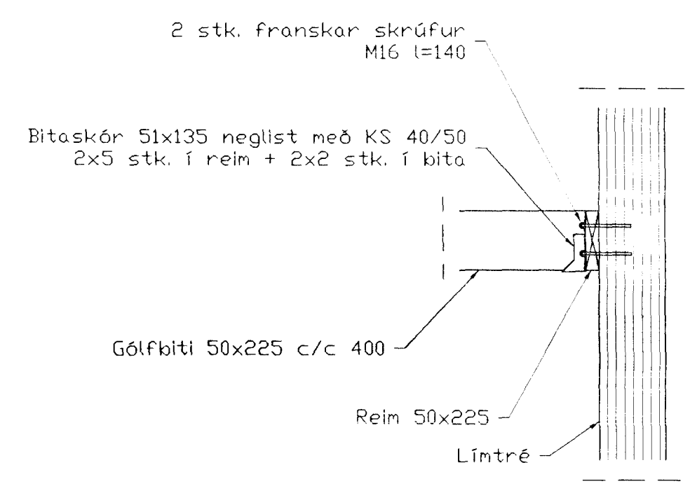
SNID 4, 1:20
