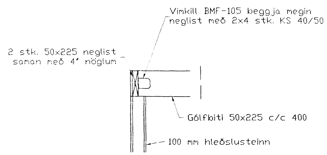
SNID 1 1:20
