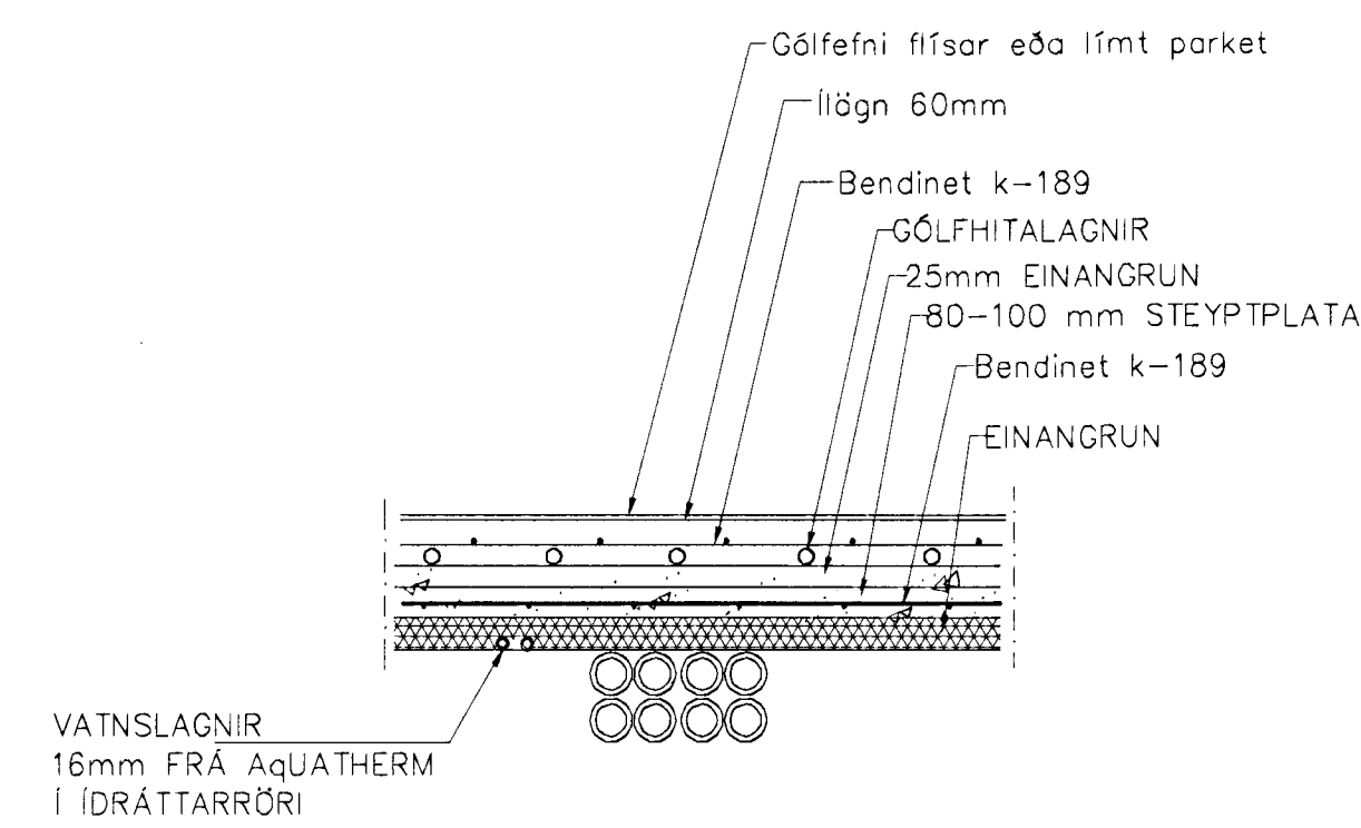
LAGNIR, SNID, 1:20
