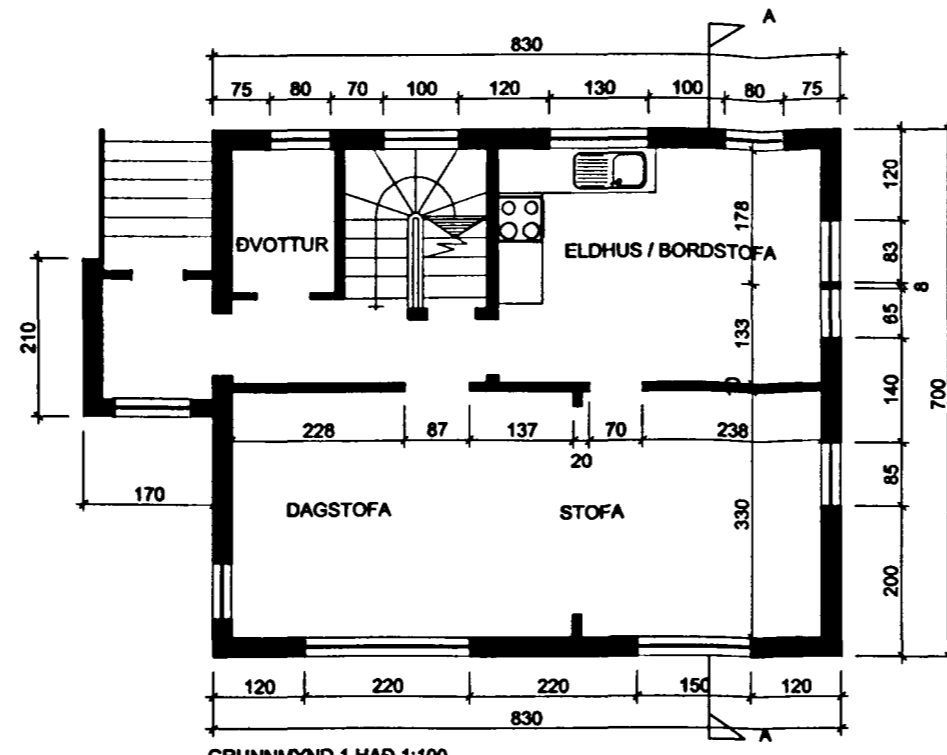
GRUNNMYND 1 HAD 1:100
