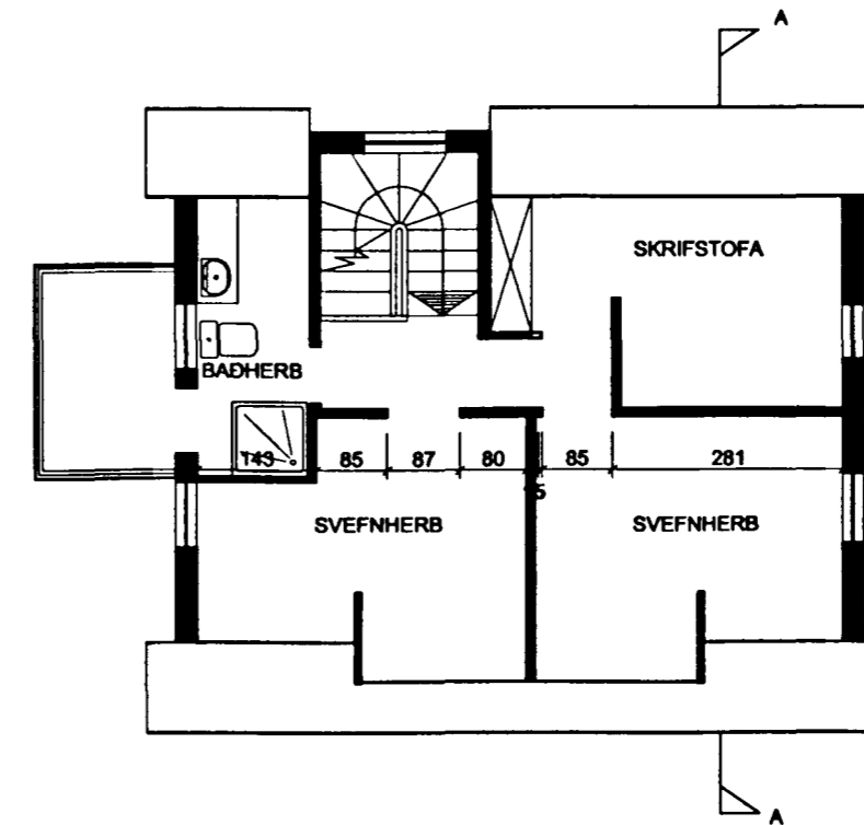
GRUNNMYND 2 HAD 1:100
