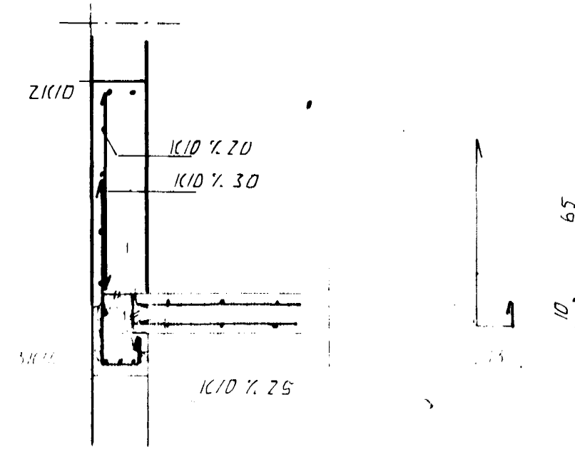
SNIB 1.1:20
