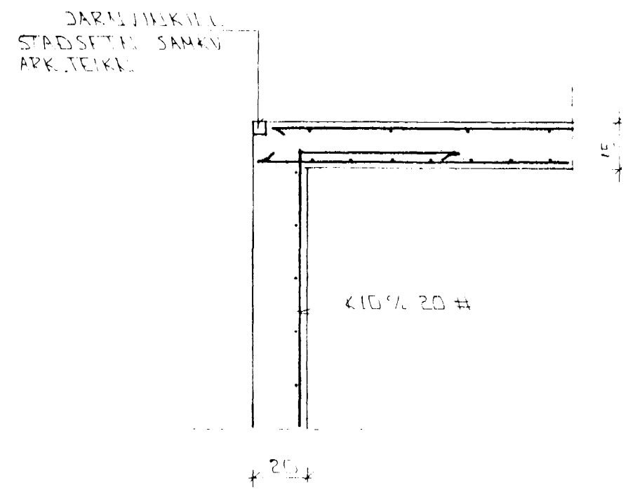
SNID 2 x 1:20
