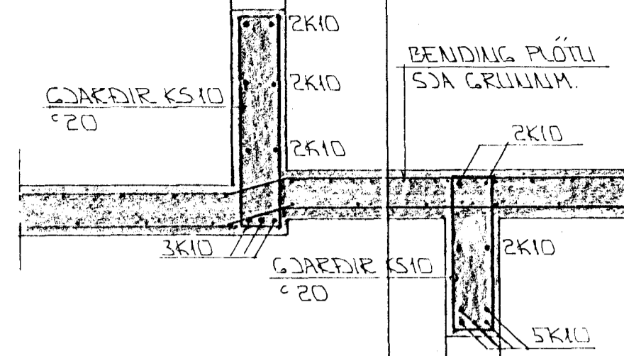
SNID 7-7 1:20
