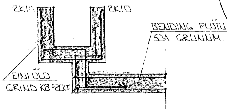
SNID 8-8 1:20
