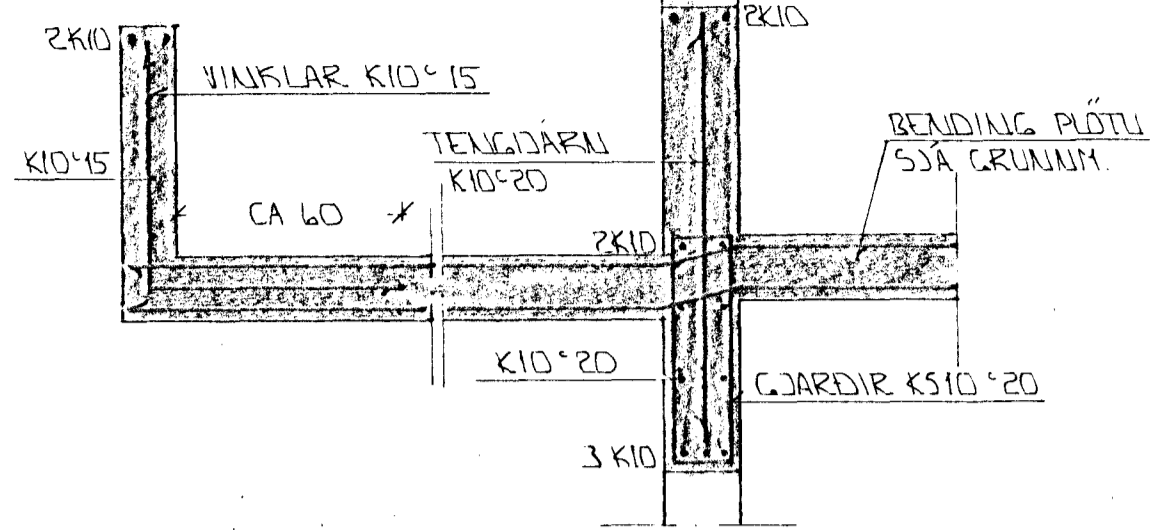
SNID 6-6 1:20
