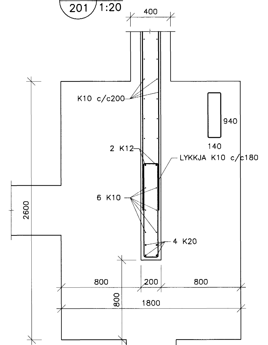
SNID G-G
