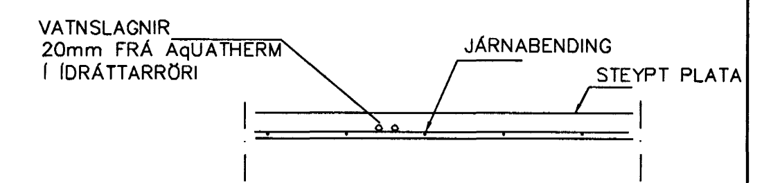
LAGNIR, SNID, 1:20
