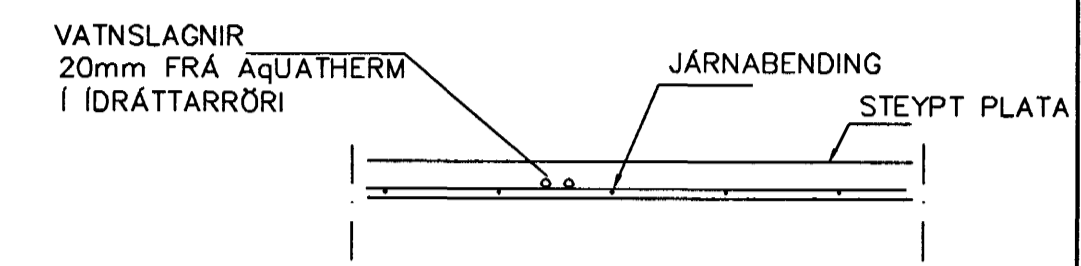
LAGNIR, SNID, 1:20
