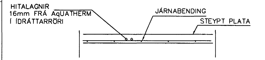
LAGNIR, SNID, 1:20
