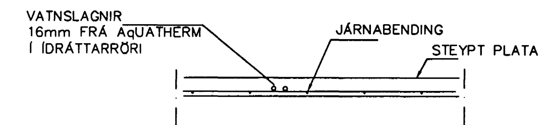
LAGNIR, SNID, 1:20
