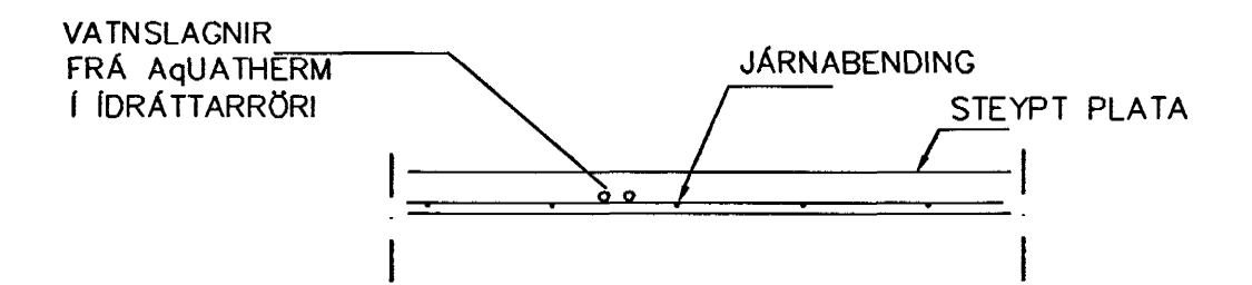
LAGNIR, SNID, 1:20
