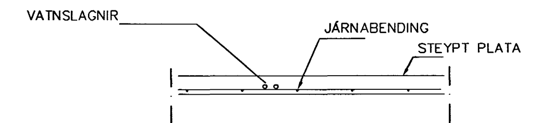
LAGNIR, SNID, 1:20
