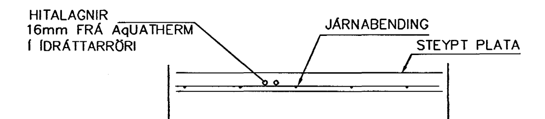
LAGNIR, SNID, 1:20
