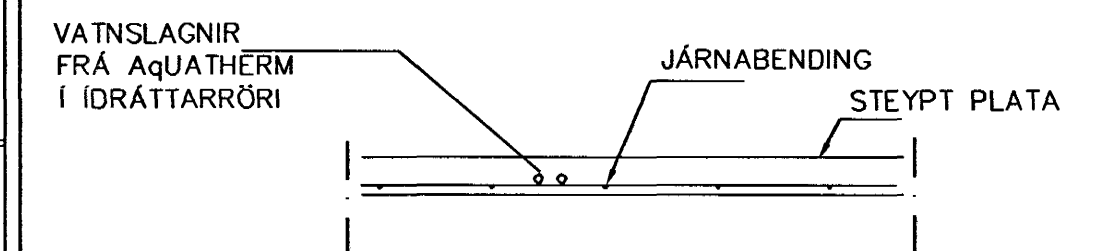
LAGNIR, SNID, 1:20
