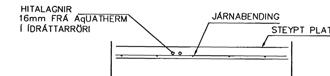
LAGNIR, SNID, 1:20
