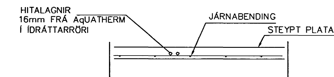
LAGNIR, SNID, 1:20
